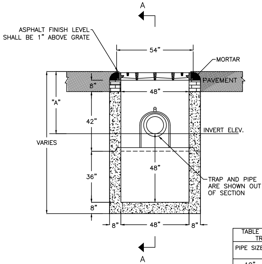
SECTIONAL ELEVATION B-B
