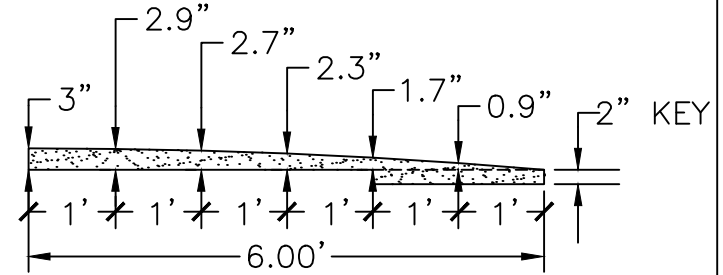
PARABOLIC SECTION - ENLARGED VIEW NTS
